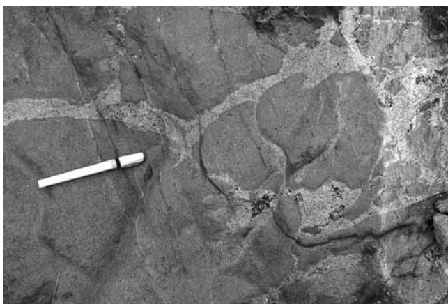
Figure 5. Commingled rock in composite dyke intruding norite of the northern unit. Note chilled margin of mafic phase against anastomosing network of coarser felsic phase containing small inclusions of hornblende norite. Pen is 13.5 cm long.
